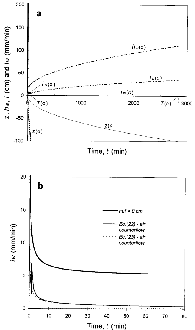
Figure 2. Prediction of equations (10), (11), (13), (14), (22), and (23) for water infiltration into a sand with parameters shown in Table 1 ( i_w is the rate of infiltration, z the depth of wetting, h_{af} the gauge air pressure ahead of the wetting front, and T the total time of infiltration at z = B = 100 cm; c and o with parenthesis denote the "air confined" condition and the "open" condition, respectively). A close-up view of i_w in Figure 2a is shown in Figure 2b.
